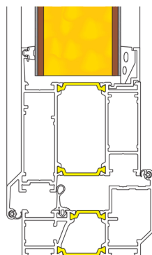
Door leaf with F1, F2, F3, F4 infill panel, see page F-38
