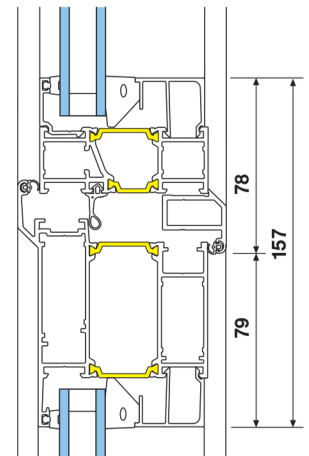
Wide sash in fixed top/side light
