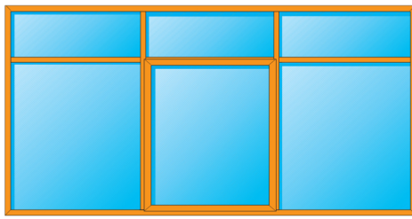
Outward opening windows with fixed side lights, or top light as an alternative
