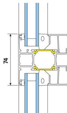
Cross-bar
