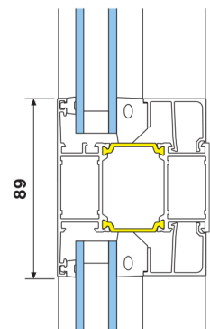
Cross-bar
