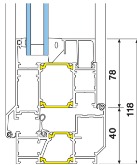
Frame with wide sash
