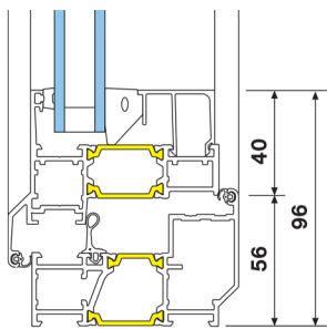
Frame with narrow sash
