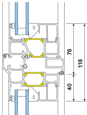
Narrow sash in fixed top/side light
