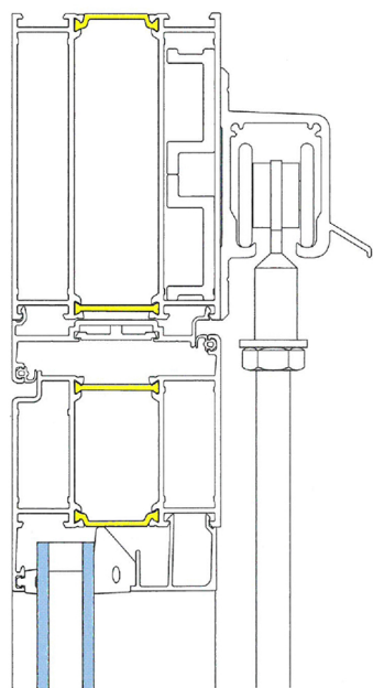
Top edge of folding door with rolling fittings
