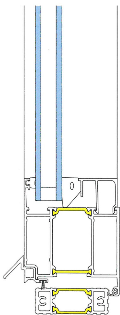
Bottom edge of folding door with a stop bead against the threshold
